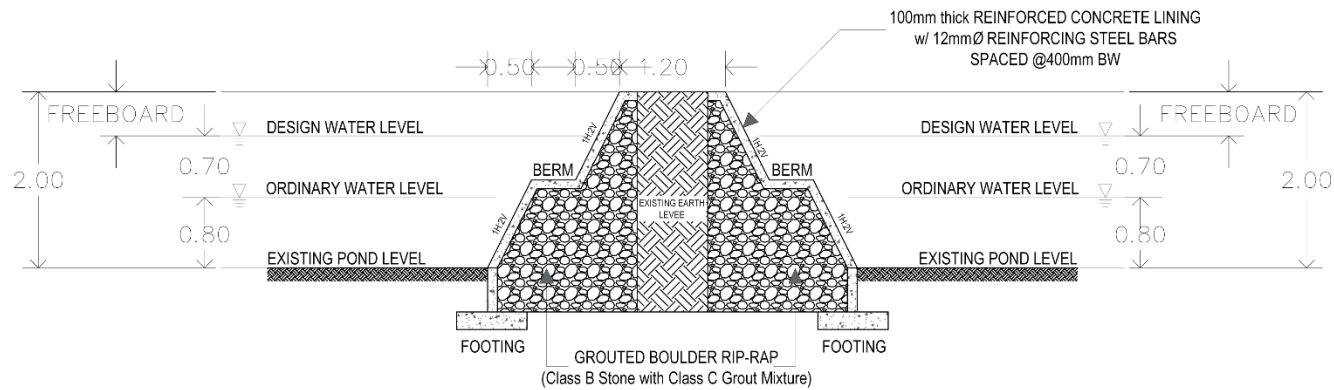
TRANSVERSE SECTION FOR DIKE B
