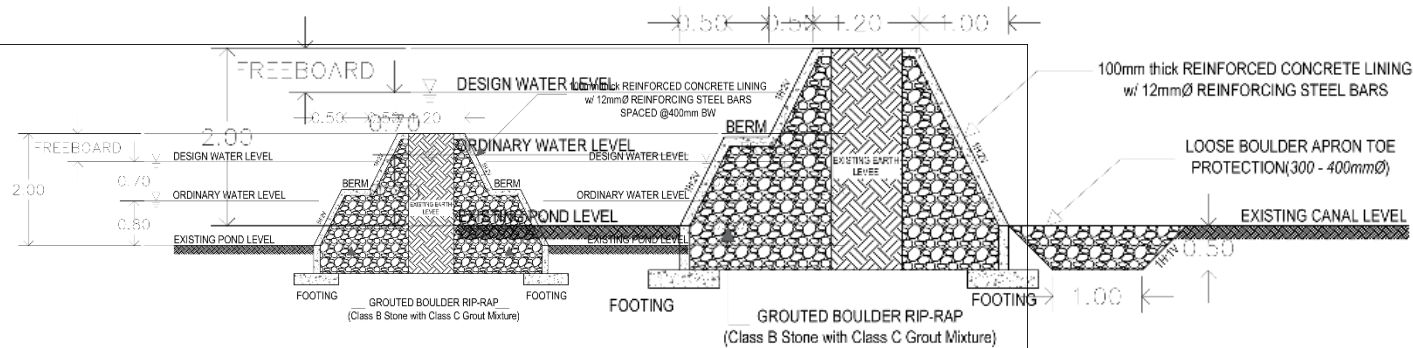
TRANSVERSE SECTION FOR DIKE B
