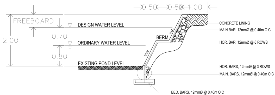
REINFORCEMENT DETAIL FOR DIKE C
