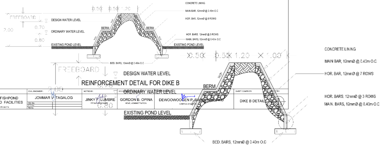
TRANSVERSE SECTION FOR DIKE A
