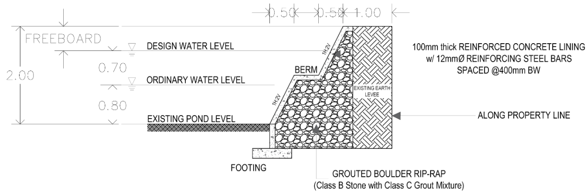
TRANSVERSE SECTION FOR DIKE C
