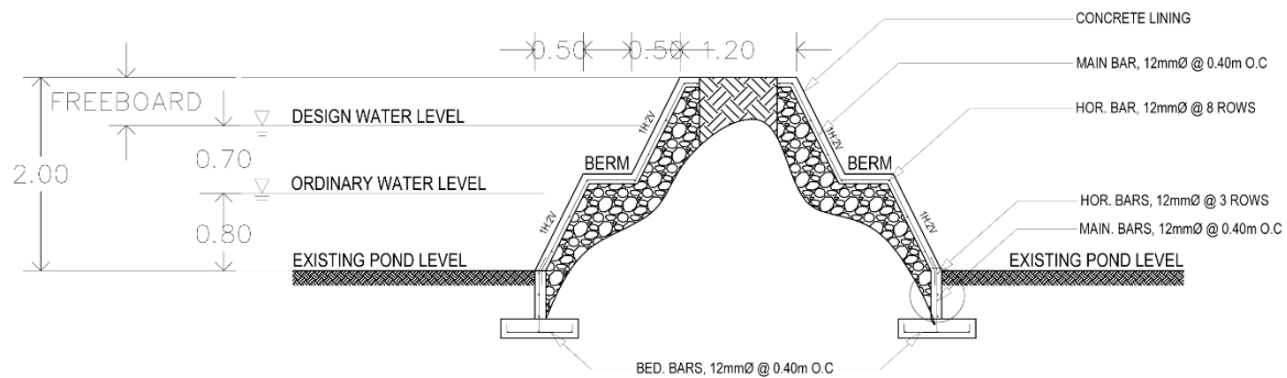
REINFORCEMENT DETAIL FOR DIKE B
